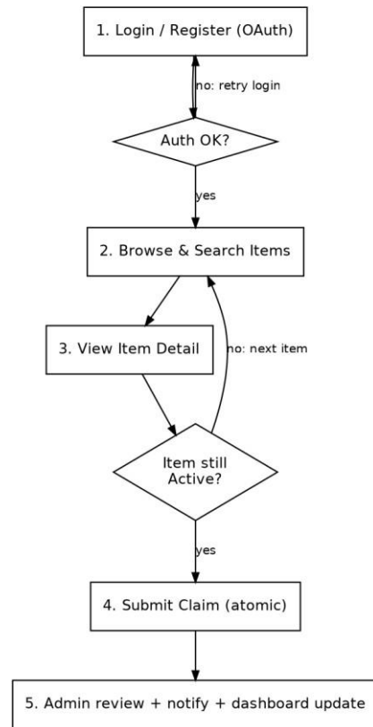
Fig. 3. UNLOST end-to-end recovery workflow with authentication and item-availability guard clauses.
